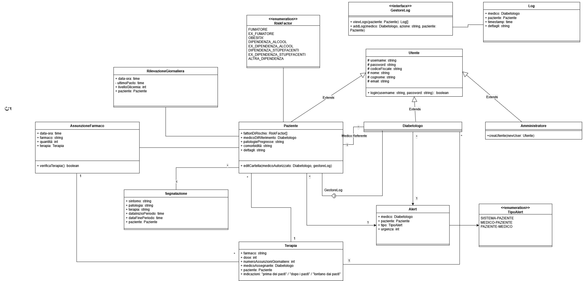
Figure 1: Class Diagram
